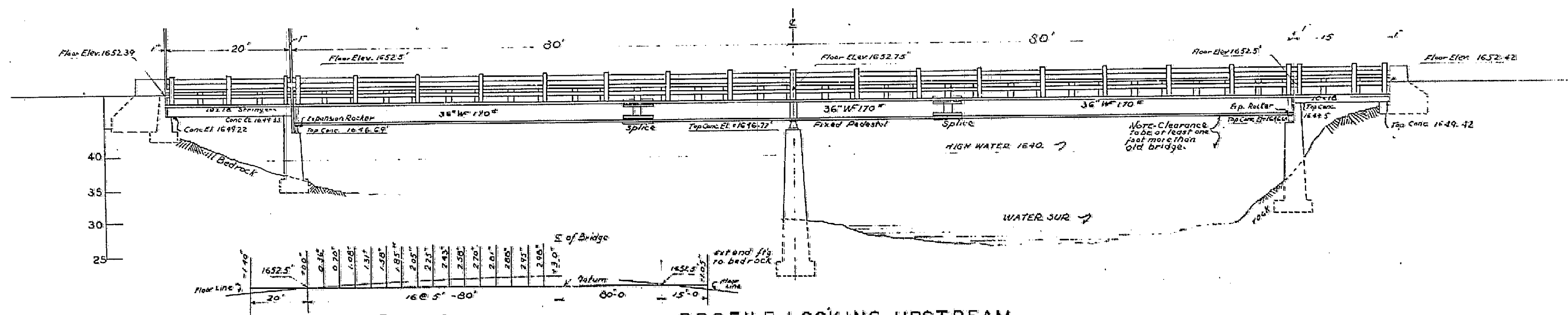
PROFILE LOOKING UPSTREAM SCALE 1" = 10'
